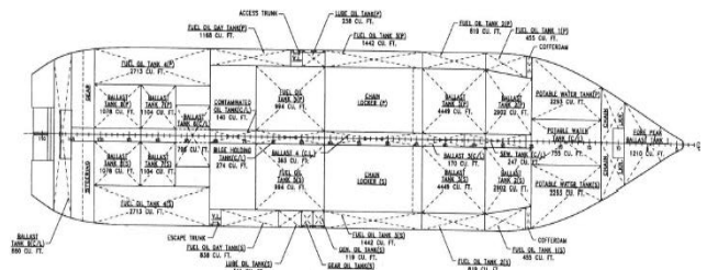
HOLD PLAN
