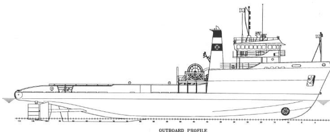
OUTBOARD PROFILE
